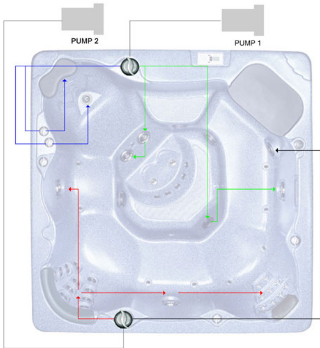
Nuage Valve Zone Diagram
